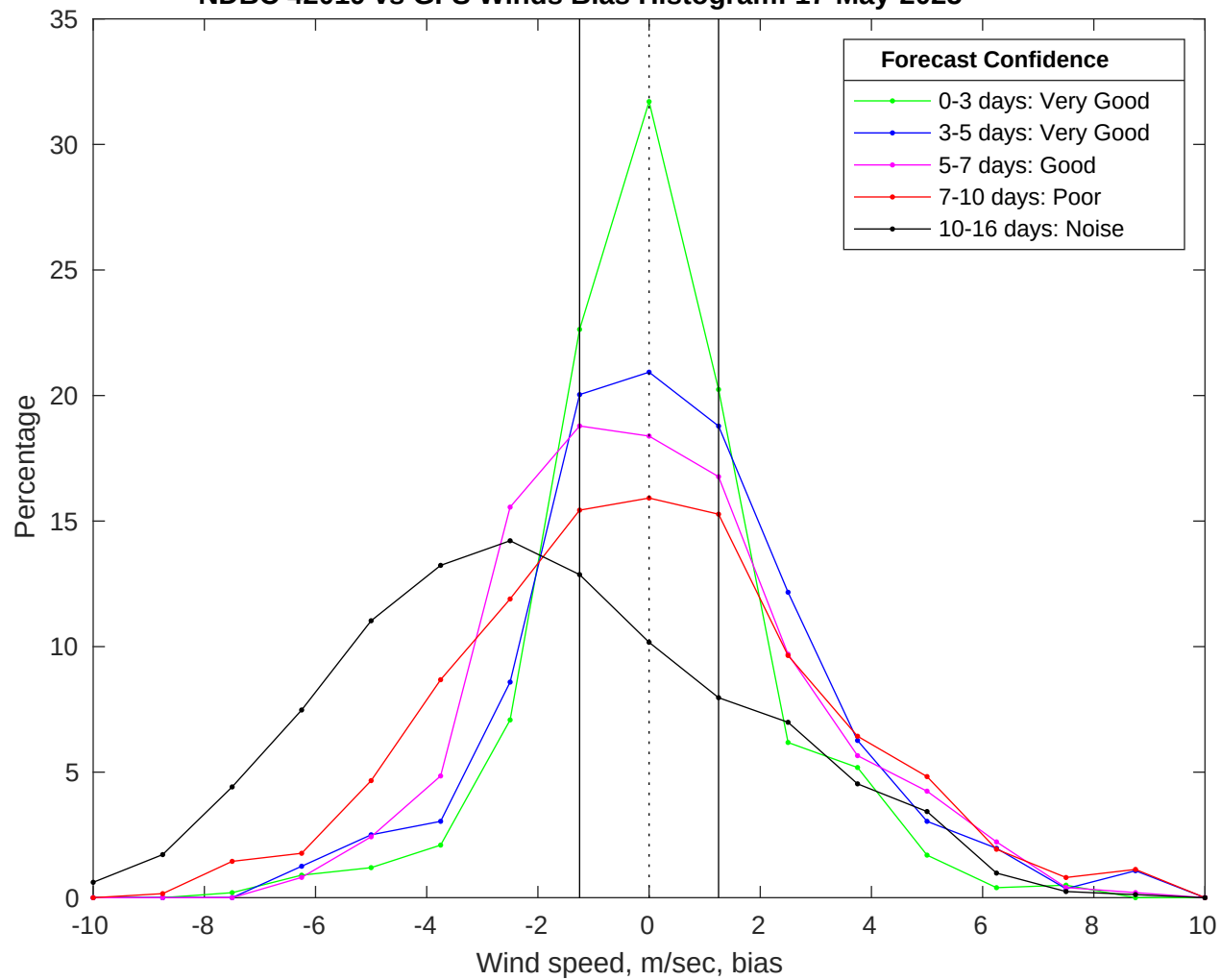
NDBC 42019 vs GFS Winds Bias Histogram: 17-May-2025
