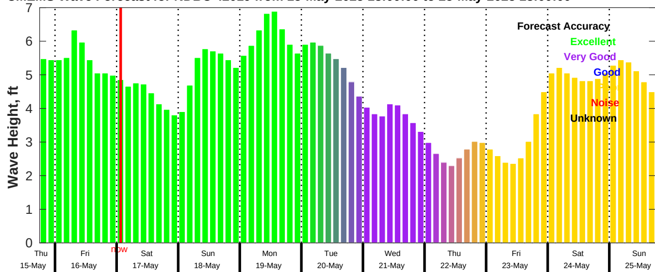
CMEMS Wave Forecast for NDBC 42019 from 15-May-2025 18:00:00 to 25-May-2025 18:00:00
