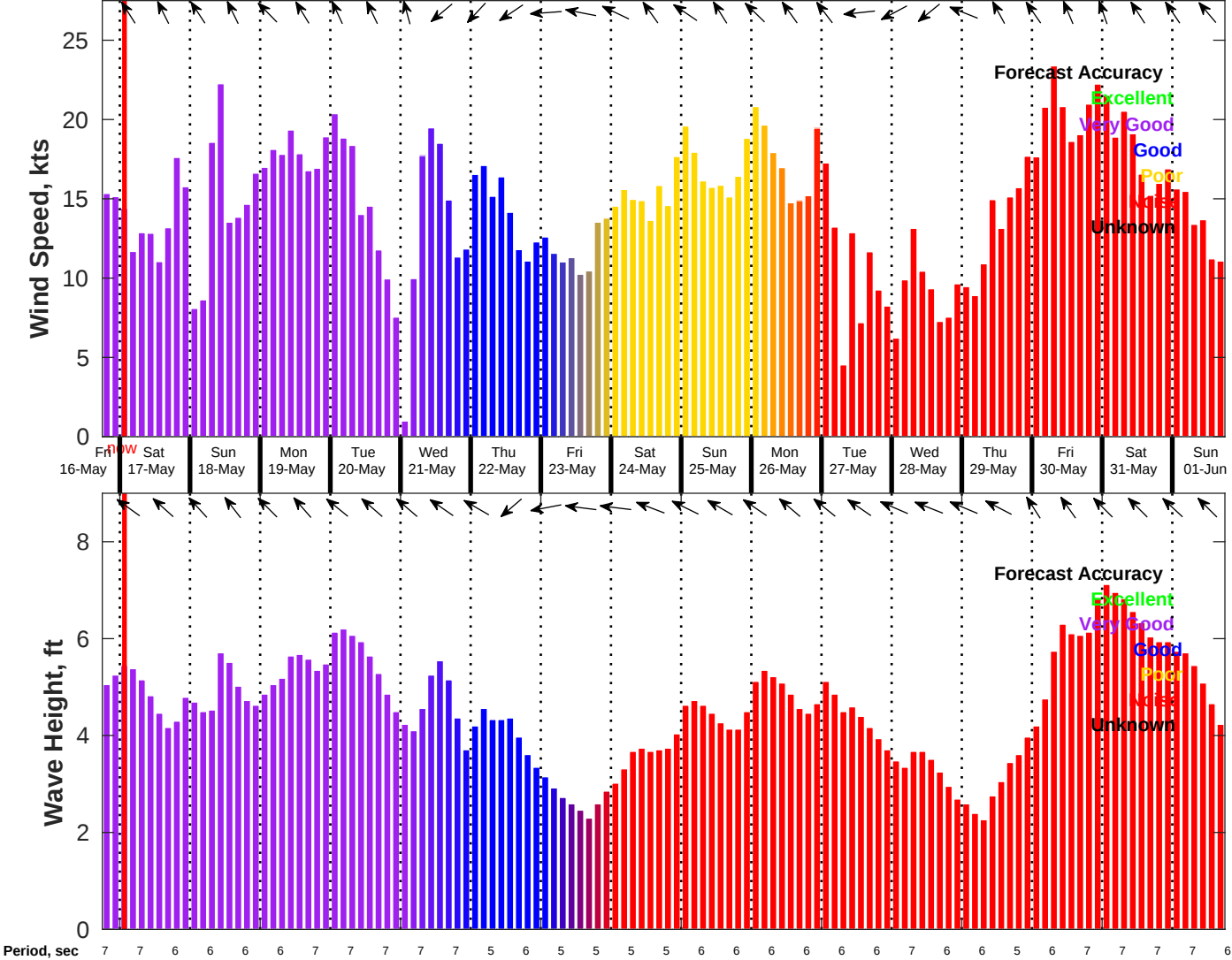
Wind & Wave Forecast for NDBC 42019 from 16-May-2025 18:00:00 to 01-Jun-2025 18:00:00
