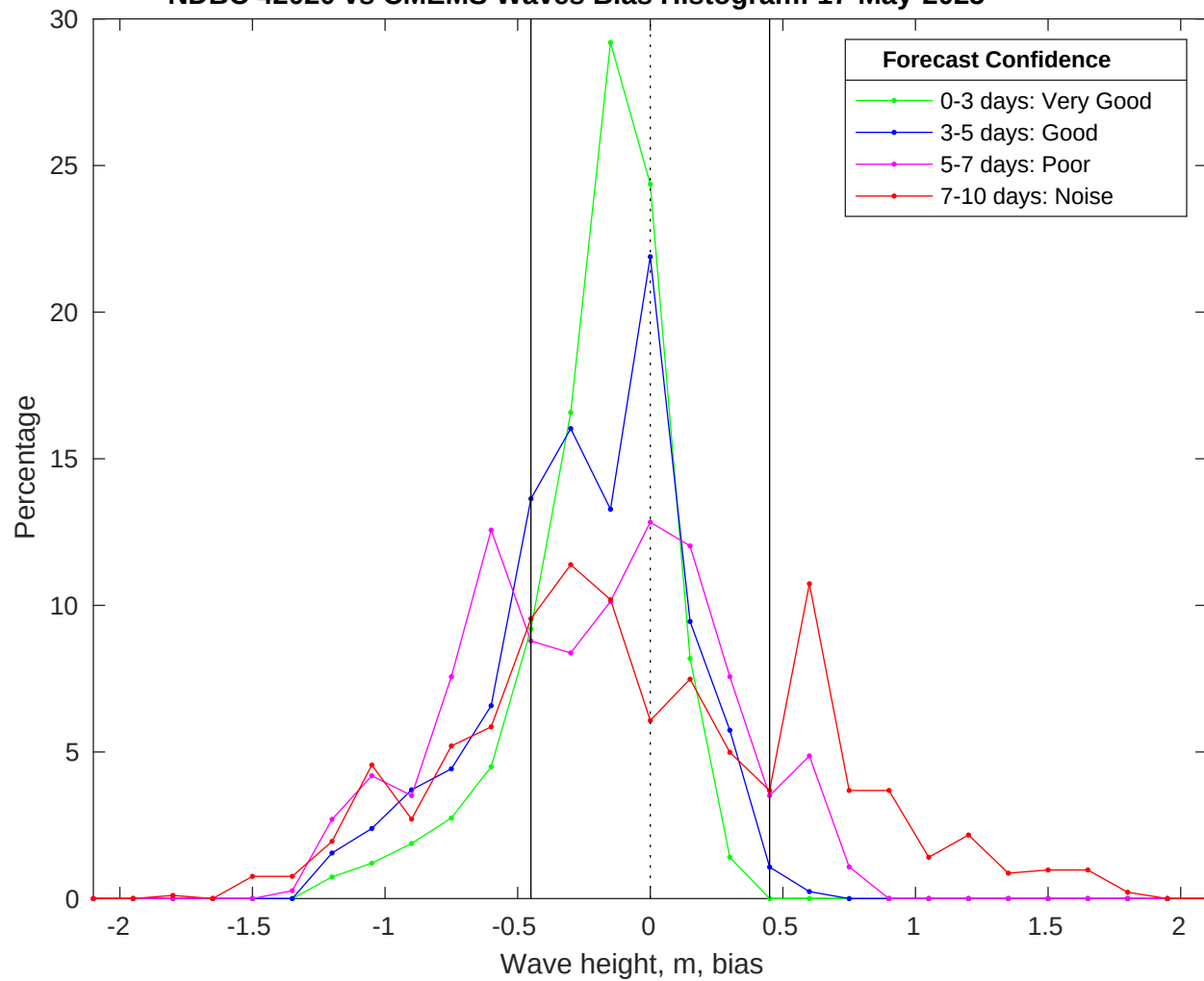
NDBC 42020 vs CMEMS Waves Bias Histogram: 17-May-2025
