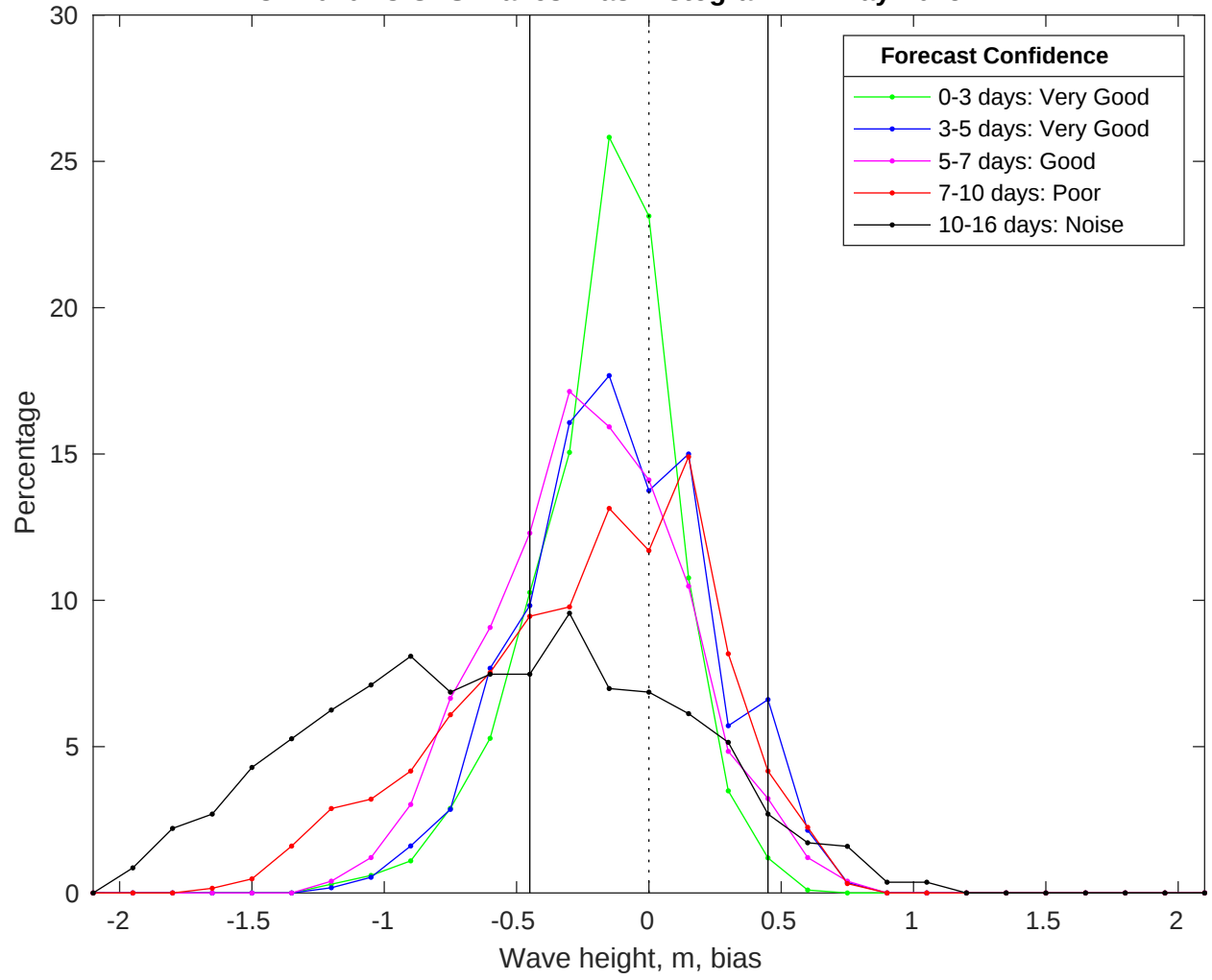
NDBC 42020 vs GFS Waves Bias Histogram: 17-May-2025
