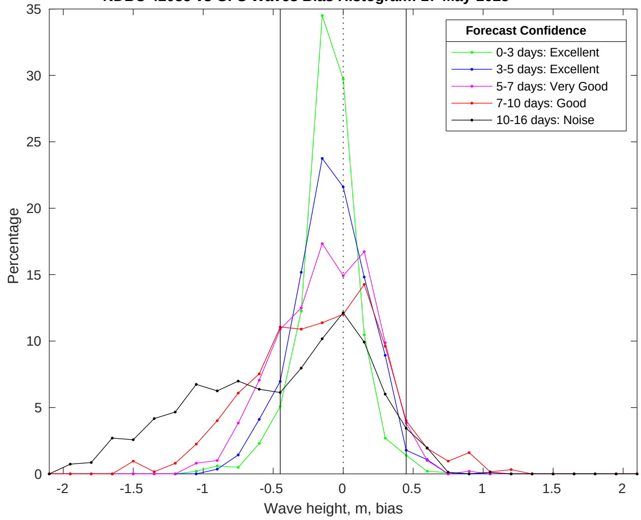
NDBC 42035 vs GFS Waves Bias Histogram: 17-May-2025
