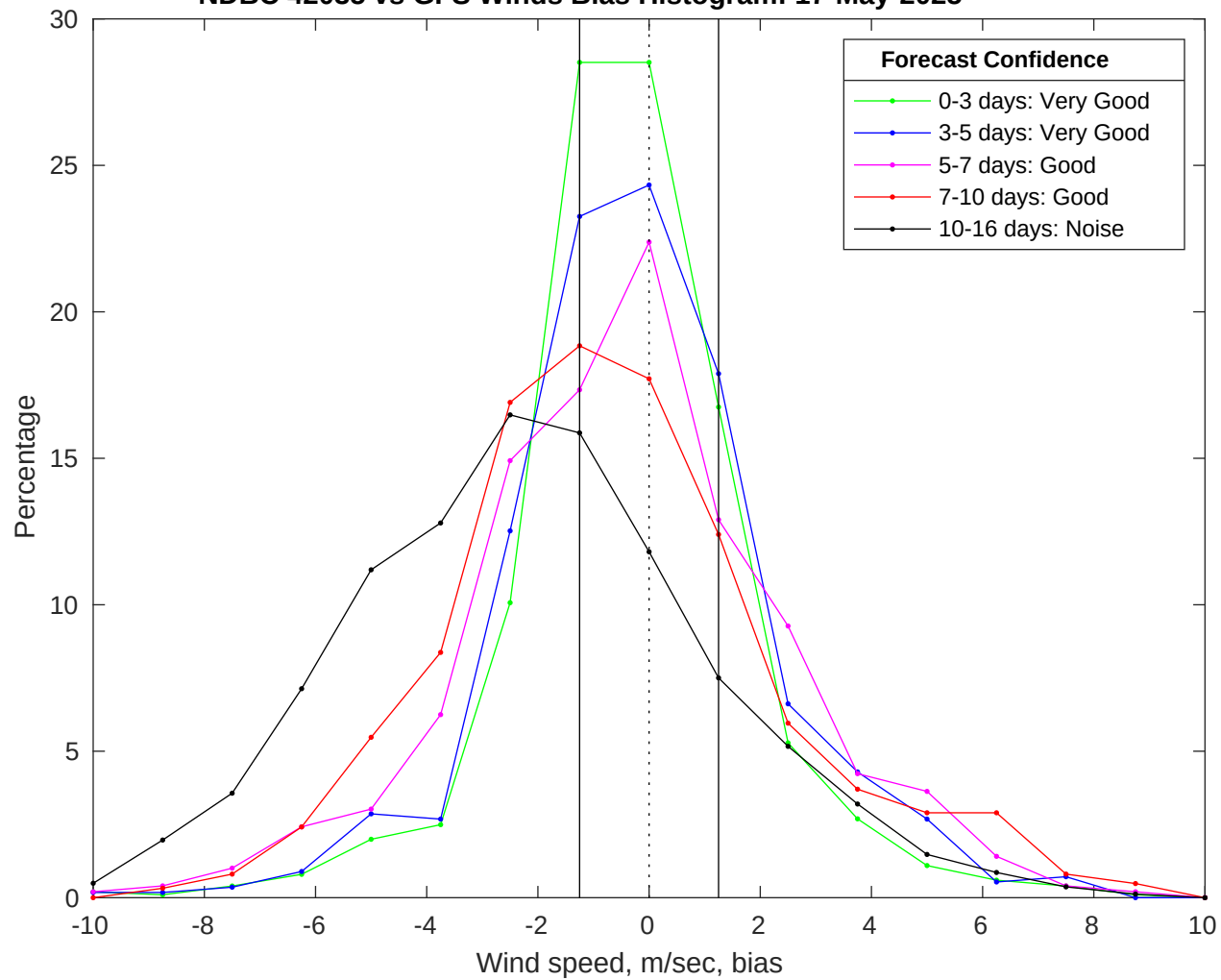
NDBC 42035 vs GFS Winds Bias Histogram: 17-May-2025
