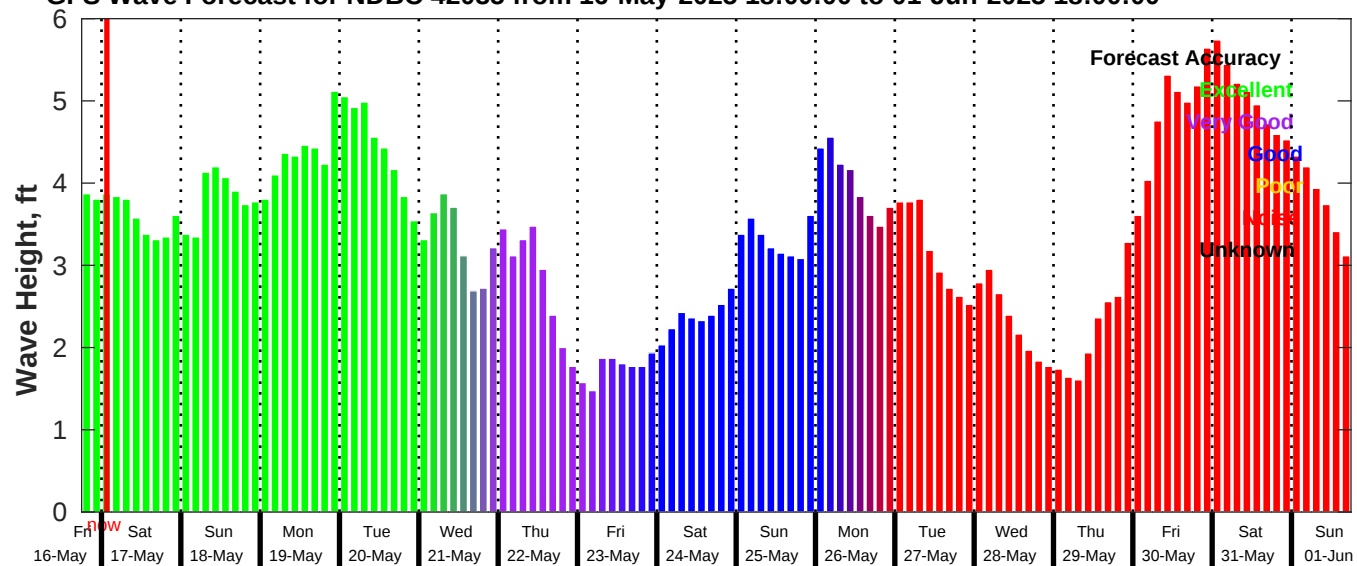
GFS Wave Forecast for NDBC 42035 from 16-May-2025 18:00:00 to 01-Jun-2025 18:00:00
