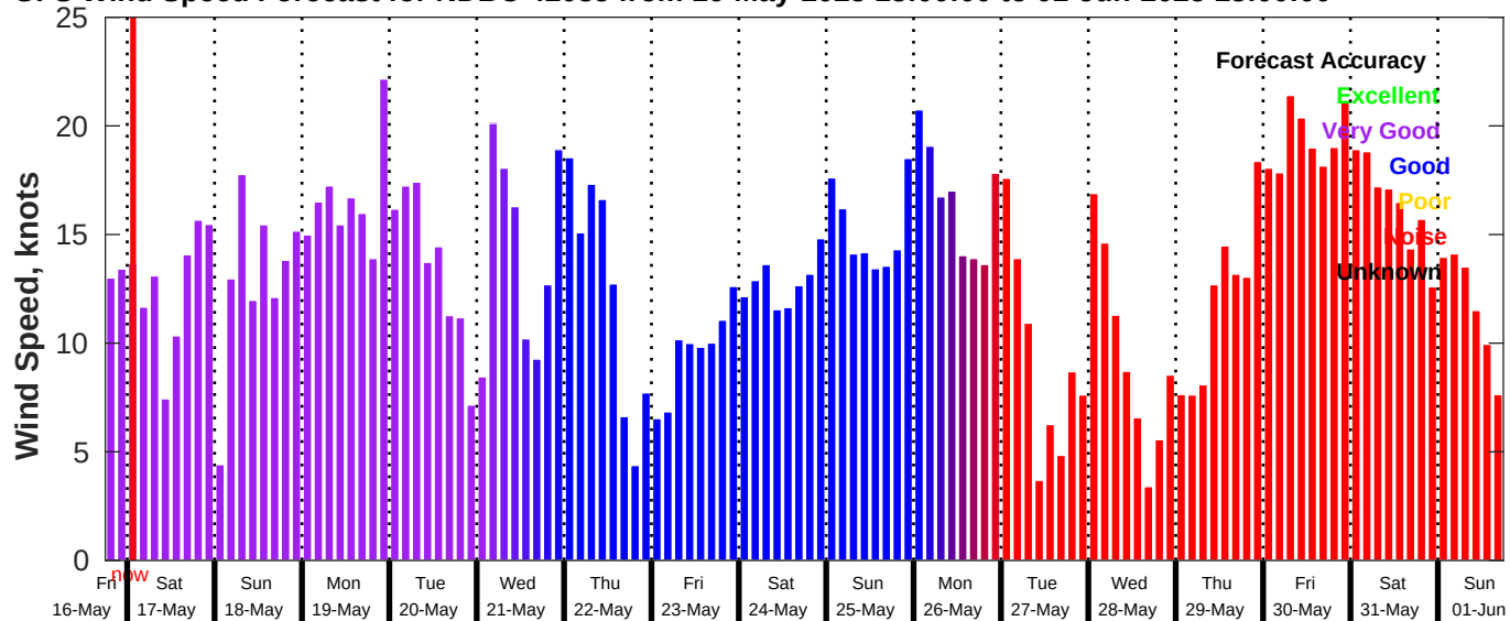
GFS Wind Speed Forecast for NDBC 42035 from 16-May-2025 18:00:00 to 01-Jun-2025 18:00:00
