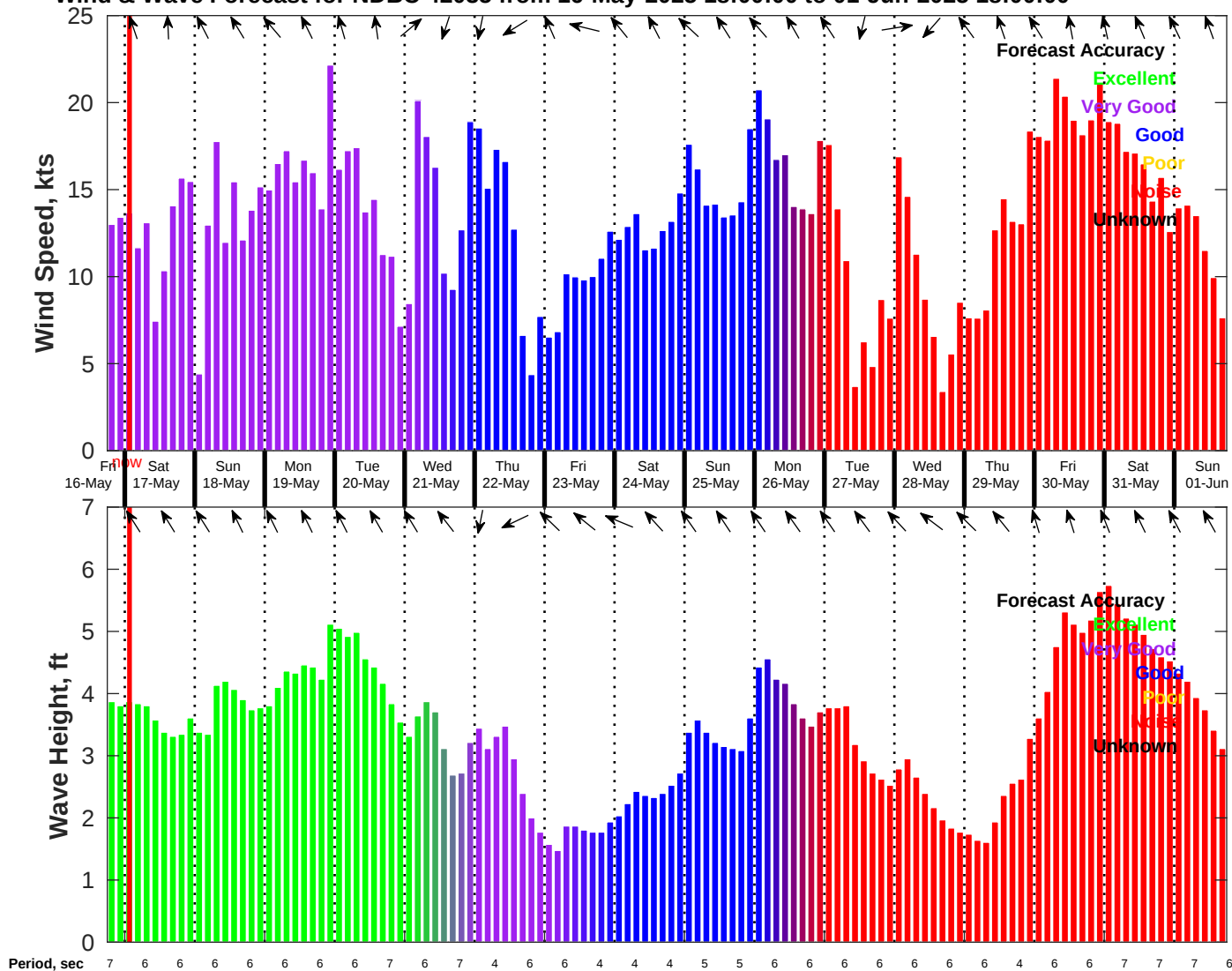
Wind & Wave Forecast for NDBC 42035 from 16-May-2025 18:00:00 to 01-Jun-2025 18:00:00
