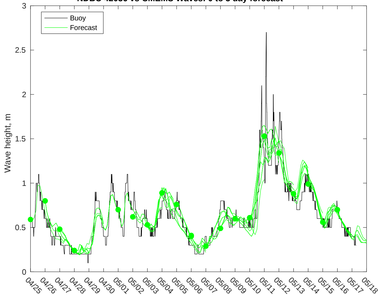
NDBC 42036 vs CMEMS Waves: 0 to 3 day forecast
