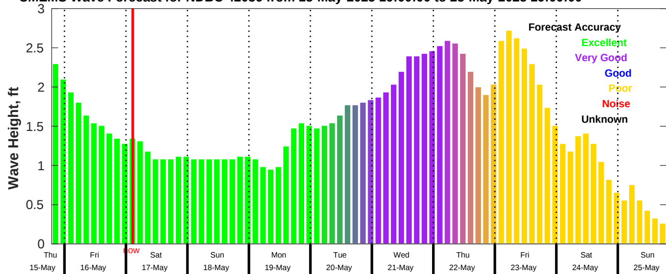
CMEMS Wave Forecast for NDBC 42036 from 15-May-2025 19:00:00 to 25-May-2025 19:00:00
