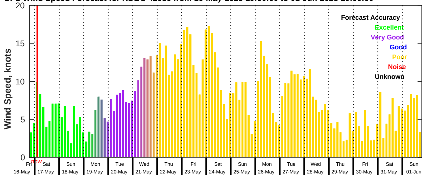
GFS Wind Speed Forecast for NDBC 42036 from 16-May-2025 19:00:00 to 01-Jun-2025 19:00:00
