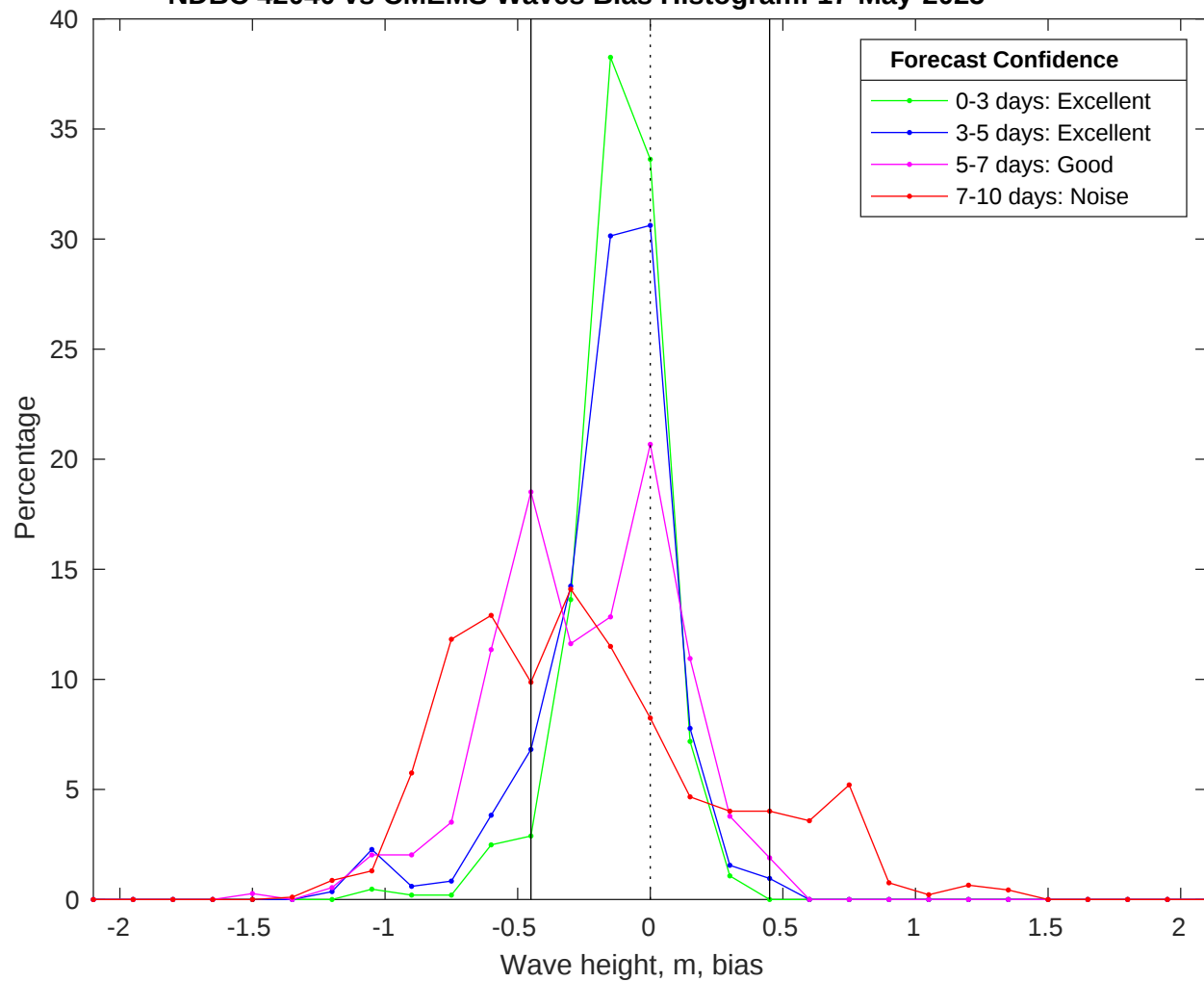
NDBC 42040 vs CMEMS Waves Bias Histogram: 17-May-2025
