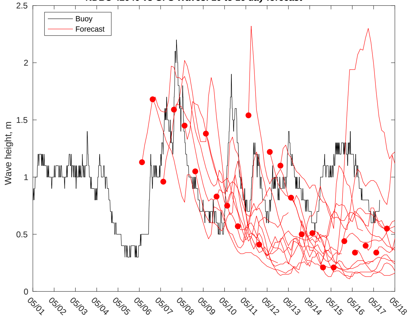
NDBC 42040 vs GFS Waves: 10 to 16 day forecast
