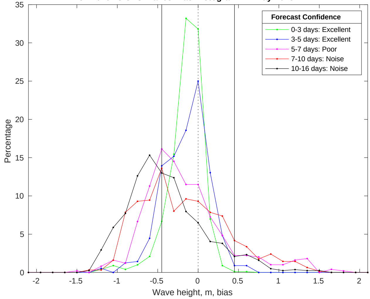
NDBC 42040 vs GFS Waves Bias Histogram: 17-May-2025
