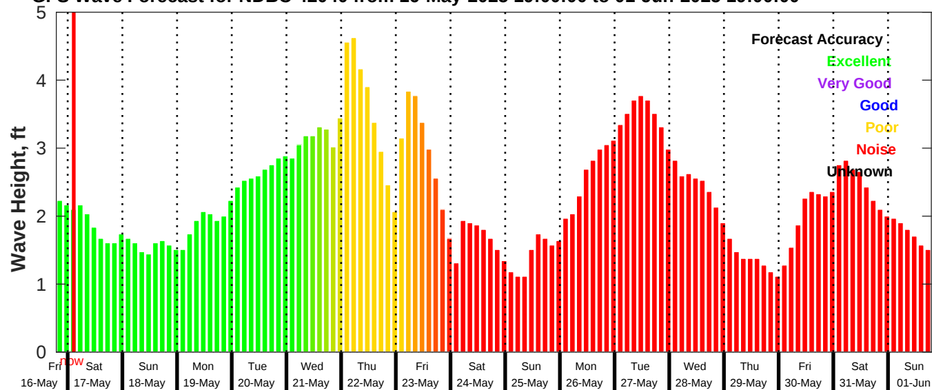
GFS Wave Forecast for NDBC 42040 from 16-May-2025 19:00:00 to 01-Jun-2025 19:00:00
