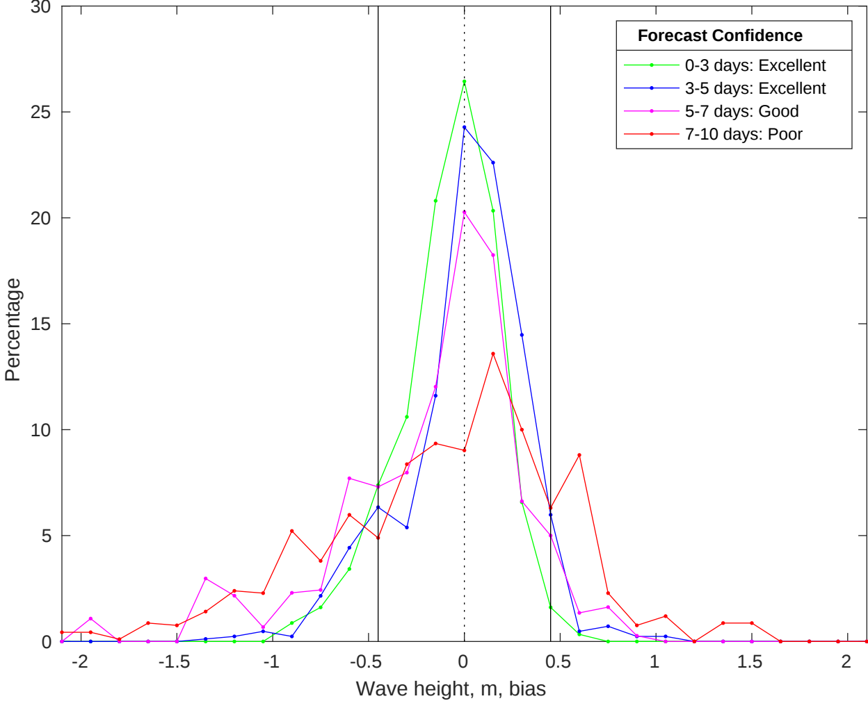
NDBC 46011 vs CMEMS Waves Bias Histogram: 17-May-2025
