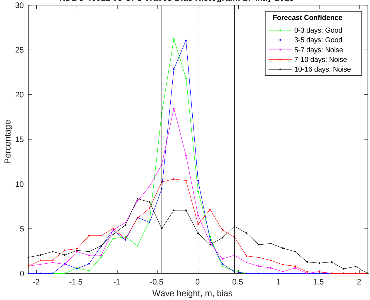
NDBC 46011 vs GFS Waves Bias Histogram: 17-May-2025
