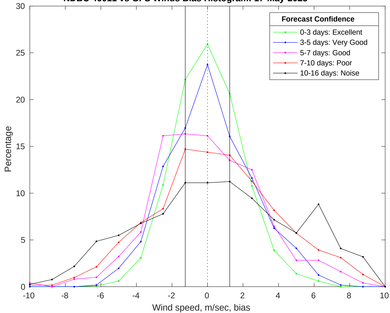
NDBC 46011 vs GFS Winds Bias Histogram: 17-May-2025
