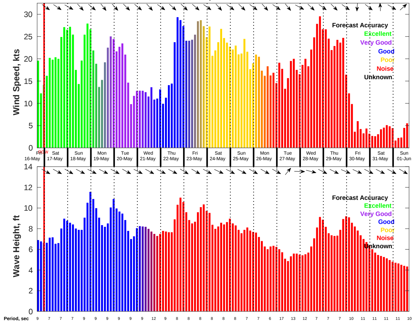
Wind & Wave Forecast for NDBC 46011 from 16-May-2025 16:00:00 to 01-Jun-2025 16:00:00
