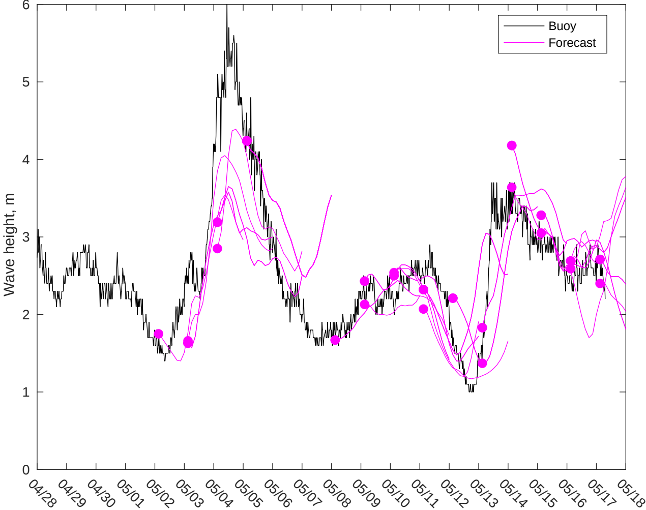
NDBC 46028 vs CMEMS Waves: 7 to 10 day forecast
