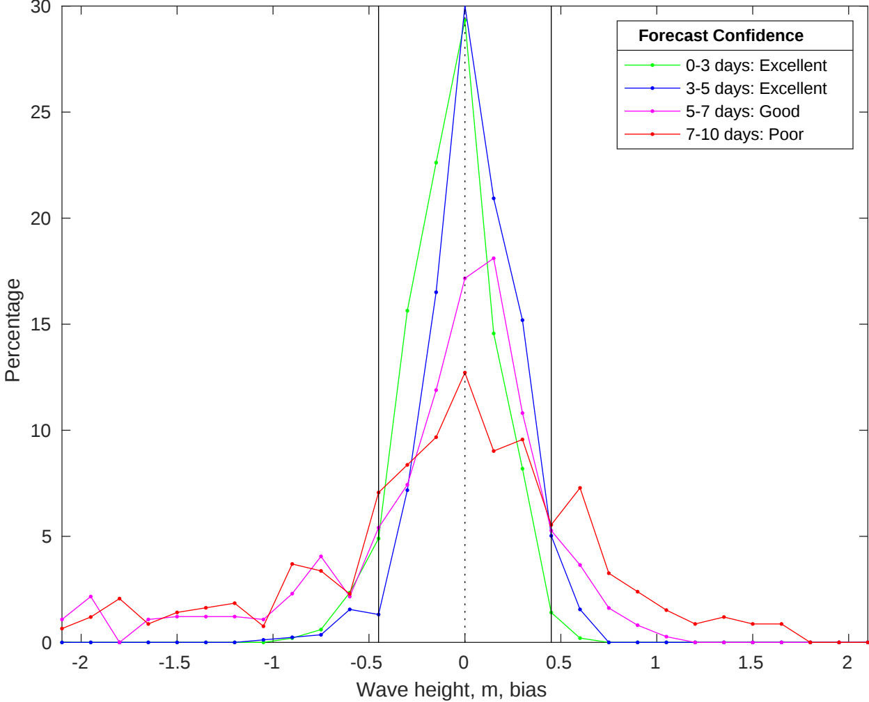
NDBC 46028 vs CMEMS Waves Bias Histogram: 17-May-2025
