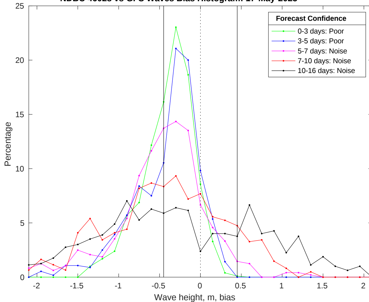
NDBC 46028 vs GFS Waves Bias Histogram: 17-May-2025
