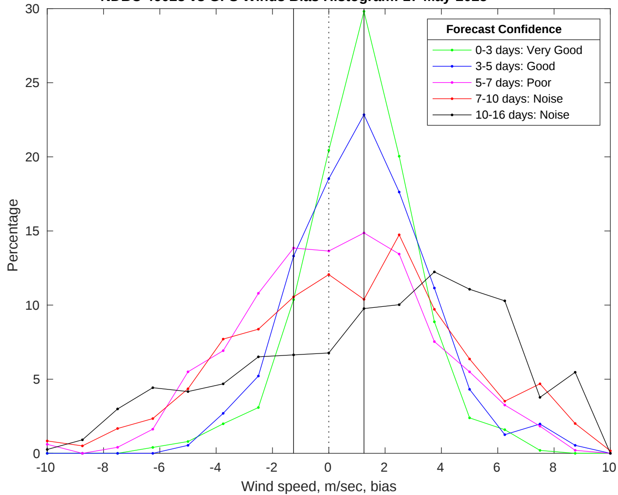
NDBC 46028 vs GFS Winds Bias Histogram: 17-May-2025
