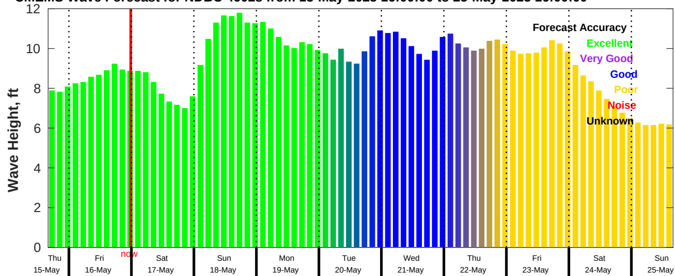
CMEMS Wave Forecast for NDBC 46028 from 15-May-2025 16:00:00 to 25-May-2025 16:00:00
