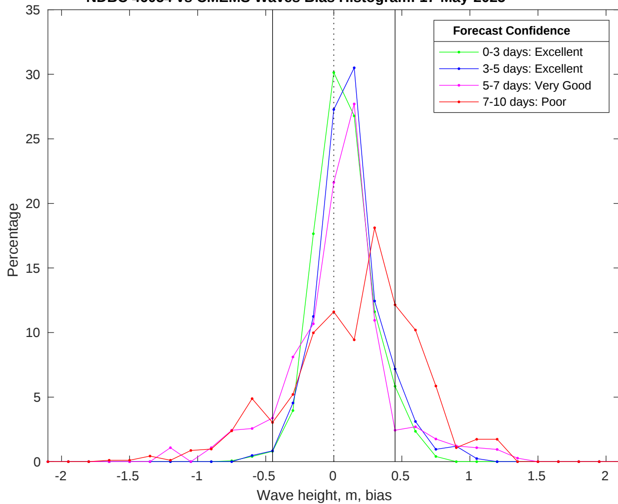
NDBC 46054 vs CMEMS Waves Bias Histogram: 17-May-2025
