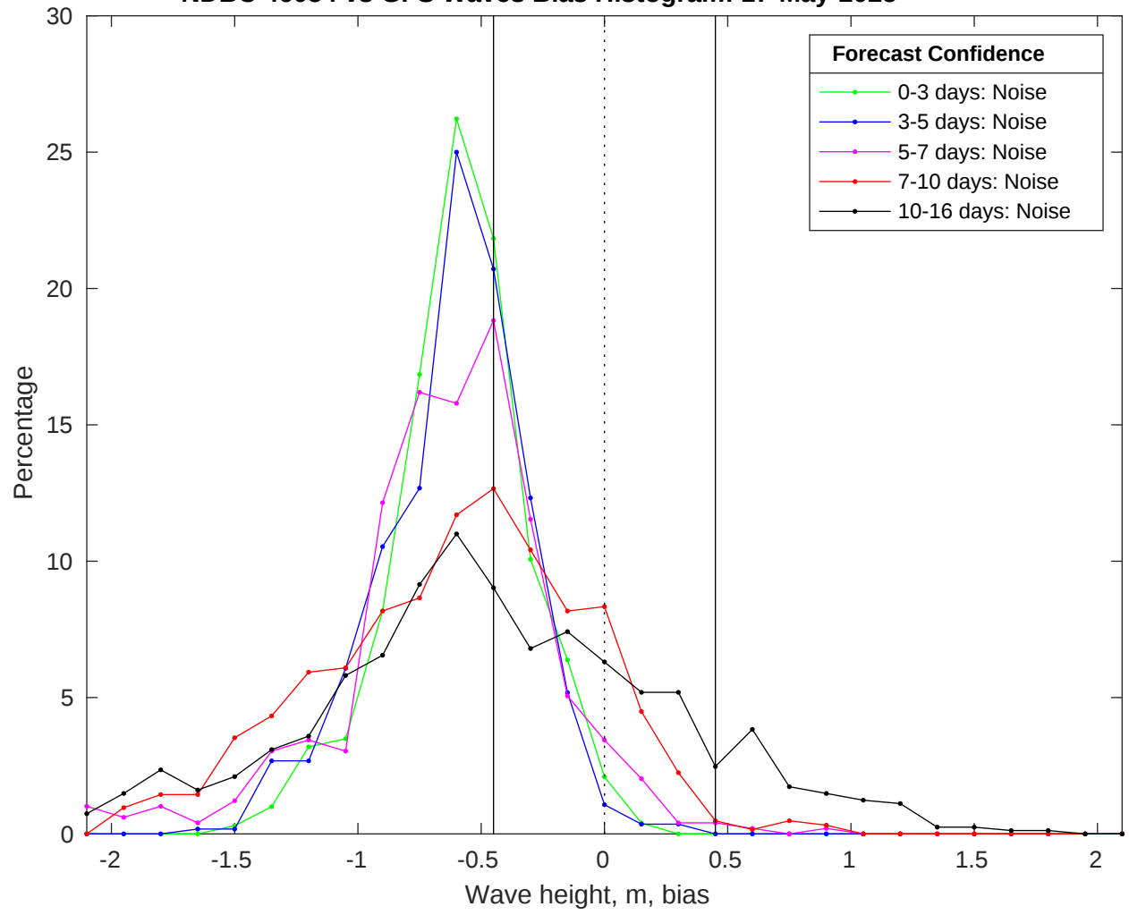
NDBC 46054 vs GFS Waves Bias Histogram: 17-May-2025
