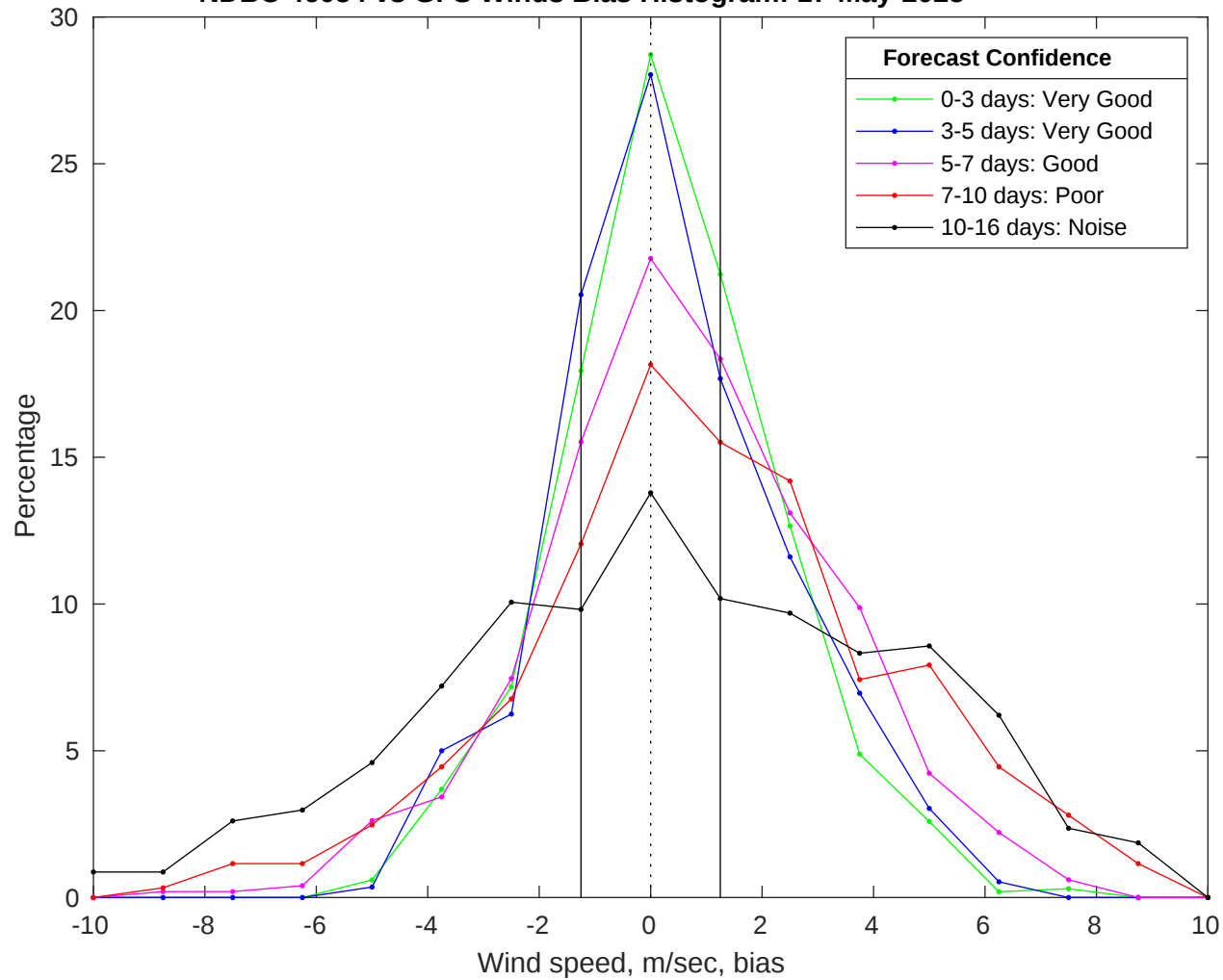
NDBC 46054 vs GFS Winds Bias Histogram: 17-May-2025
