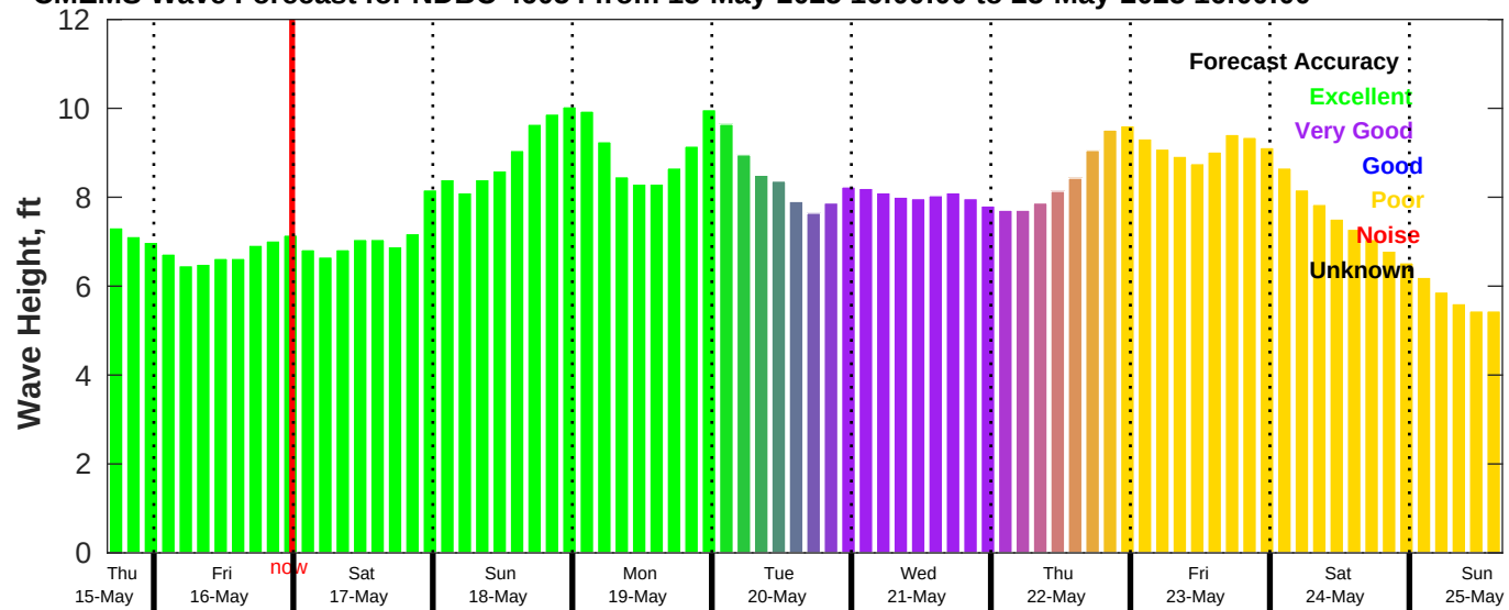
CMEMS Wave Forecast for NDBC 46054 from 15-May-2025 16:00:00 to 25-May-2025 16:00:00
