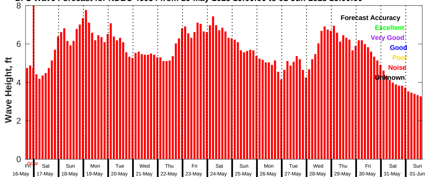
GFS Wave Forecast for NDBC 46054 from 16-May-2025 16:00:00 to 01-Jun-2025 16:00:00
