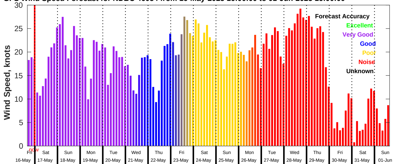
GFS Wind Speed Forecast for NDBC 46054 from 16-May-2025 16:00:00 to 01-Jun-2025 16:00:00
