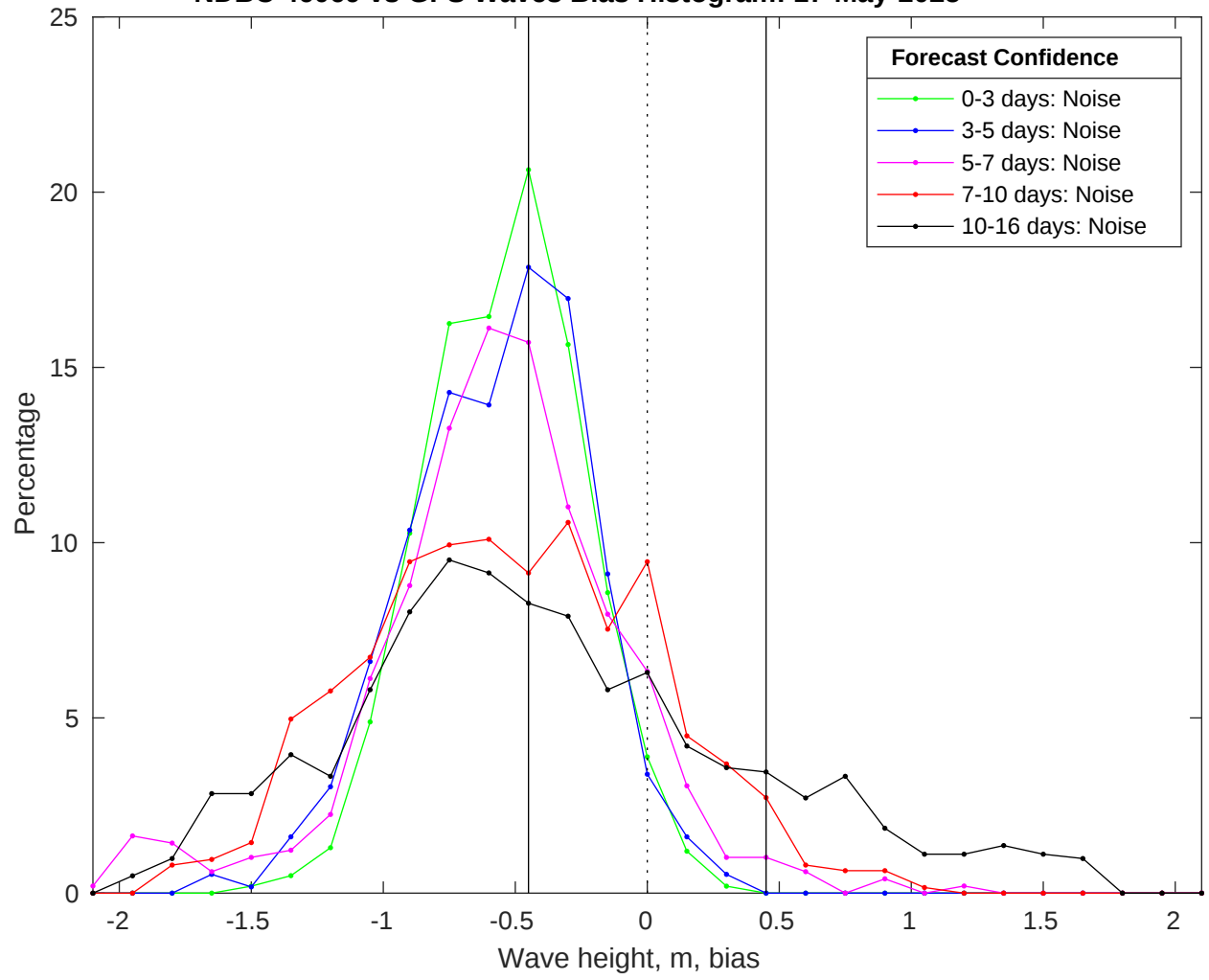
NDBC 46069 vs GFS Waves Bias Histogram: 17-May-2025
