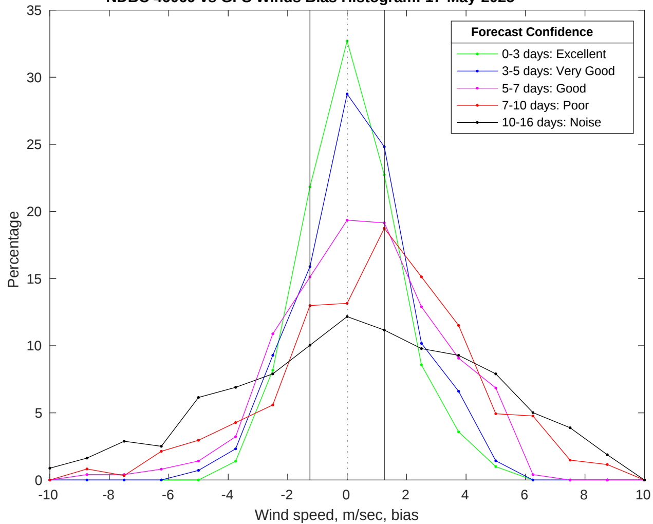
NDBC 46069 vs GFS Winds Bias Histogram: 17-May-2025
