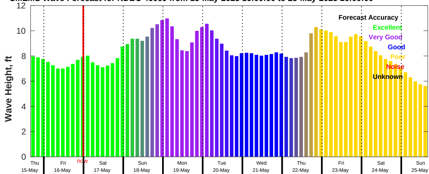
CMEMS Wave Forecast for NDBC 46069 from 15-May-2025 16:00:00 to 25-May-2025 16:00:00
