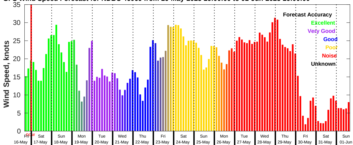
GFS Wind Speed Forecast for NDBC 46069 from 16-May-2025 16:00:00 to 01-Jun-2025 16:00:00
