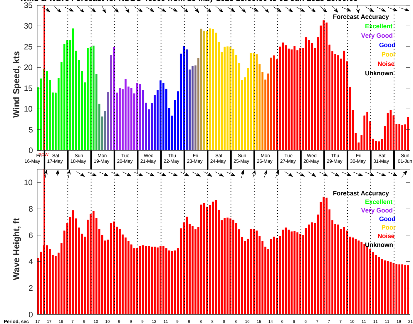
Wind & Wave Forecast for NDBC 46069 from 16-May-2025 16:00:00 to 01-Jun-2025 16:00:00
