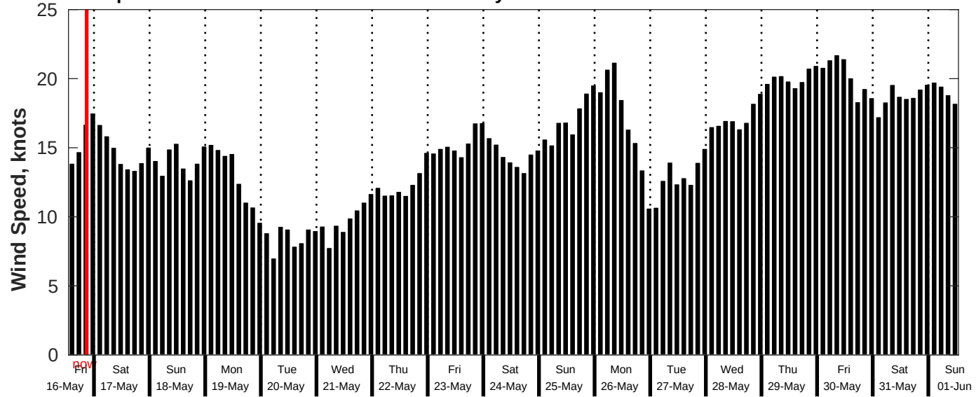
GFS Wind Speed Forecast for NDBC 51209 from 16-May-2025 13:00:00 to 01-Jun-2025 13:00:00
