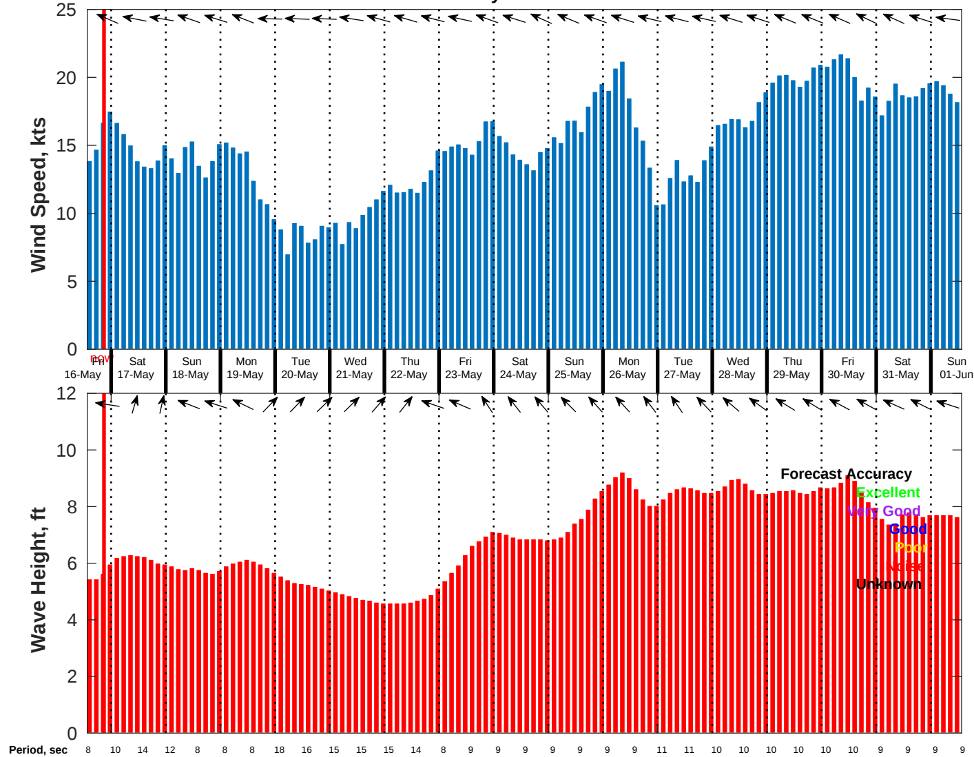
Wind & Wave Forecast for NDBC 51209 from 16-May-2025 13:00:00 to 01-Jun-2025 13:00:00
