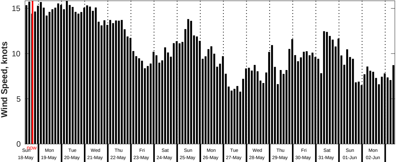
GFS Wind Speed Forecast for NDBC 52211 from 17-May-2025 10:00:00 to 02-Jun-2025 10:00:00
