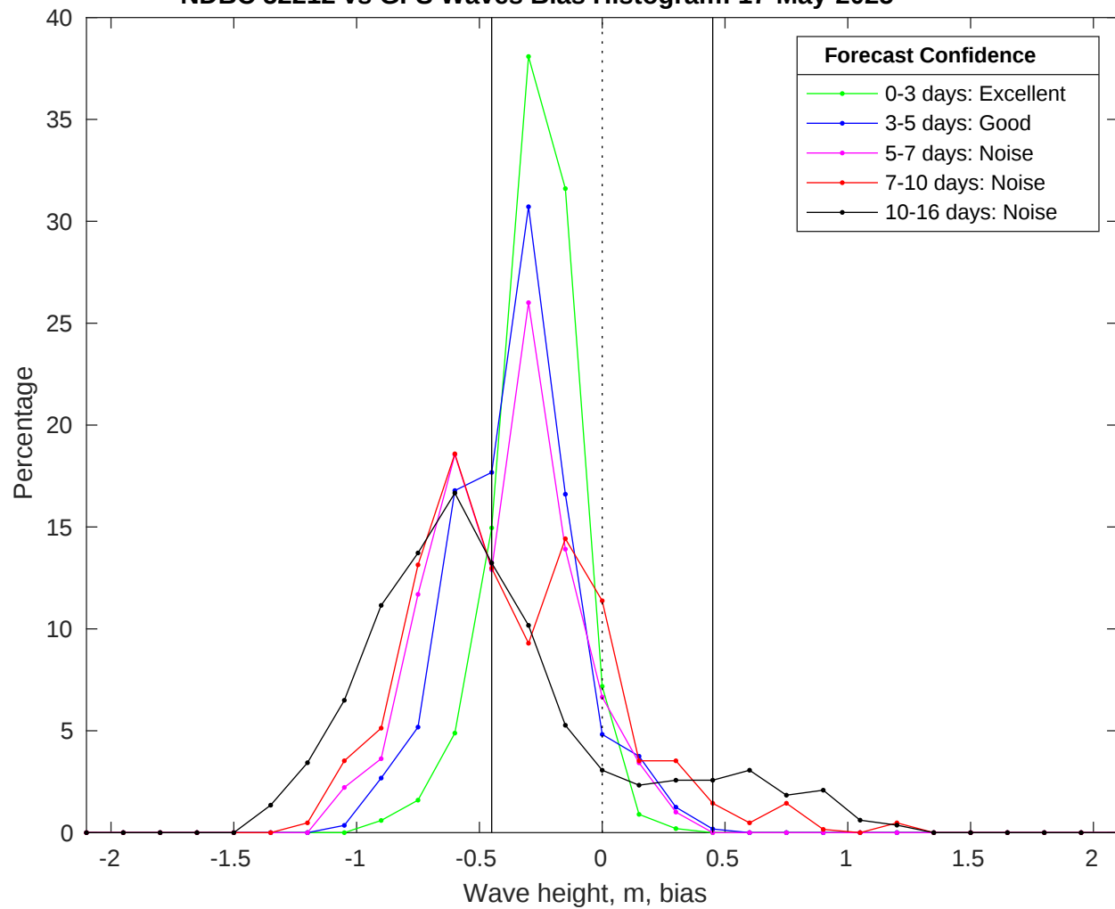
NDBC 52212 vs GFS Waves Bias Histogram: 17-May-2025
