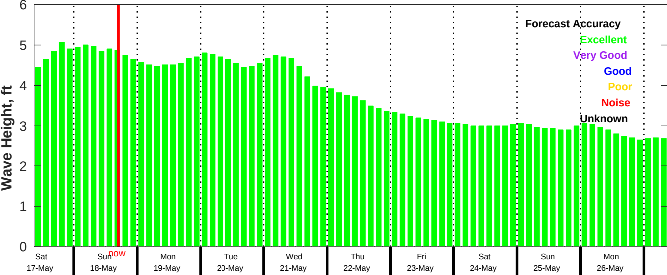
CMEMS Wave Forecast for NDBC 52212 from 16-May-2025 09:00:00 to 26-May-2025 09:00:00
