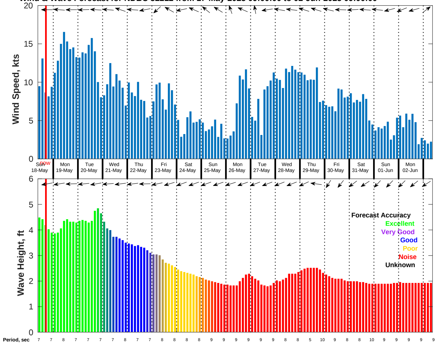
Wind & Wave Forecast for NDBC 52212 from 17-May-2025 09:00:00 to 02-Jun-2025 09:00:00
