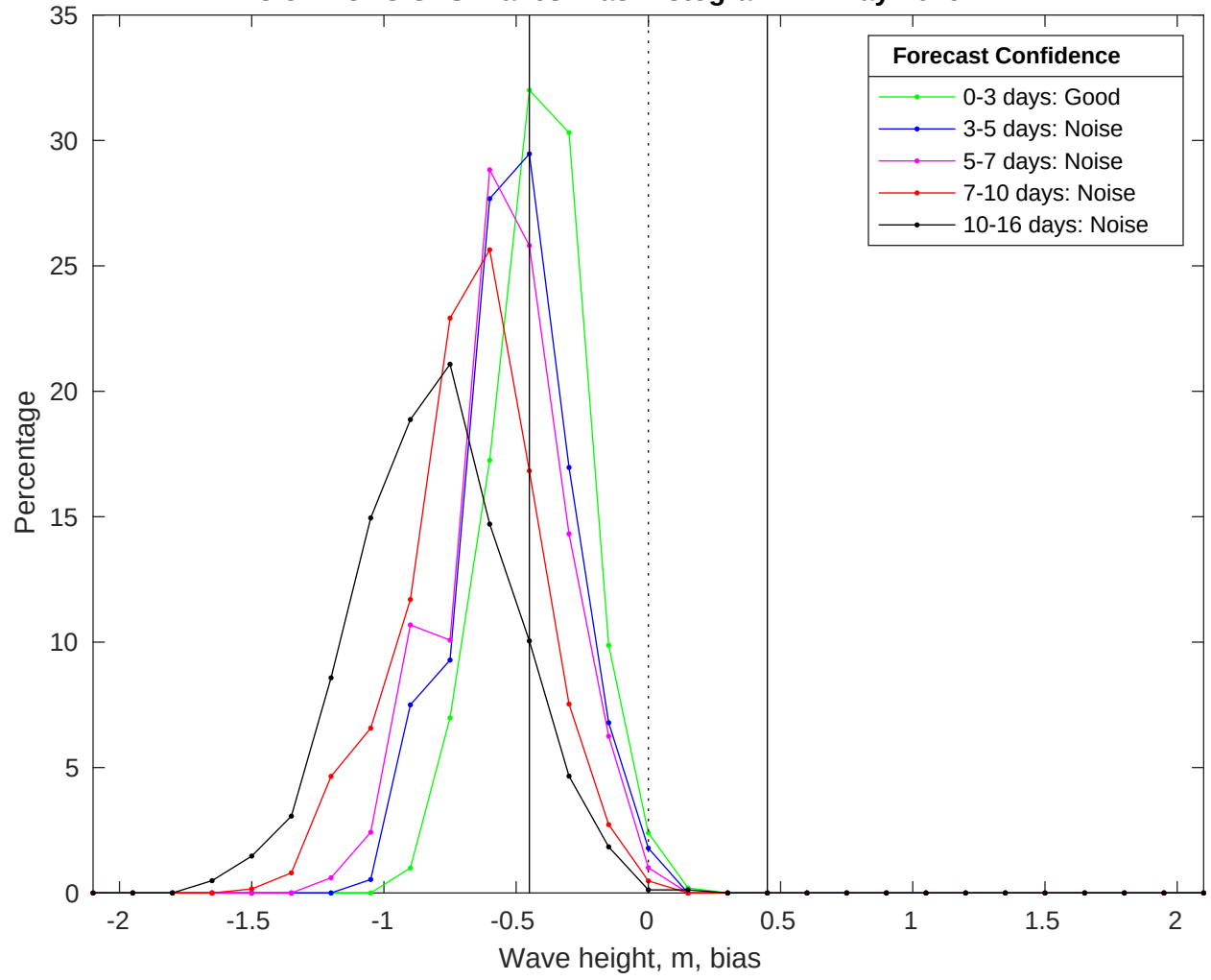
NDBC 52213 vs GFS Waves Bias Histogram: 17-May-2025
