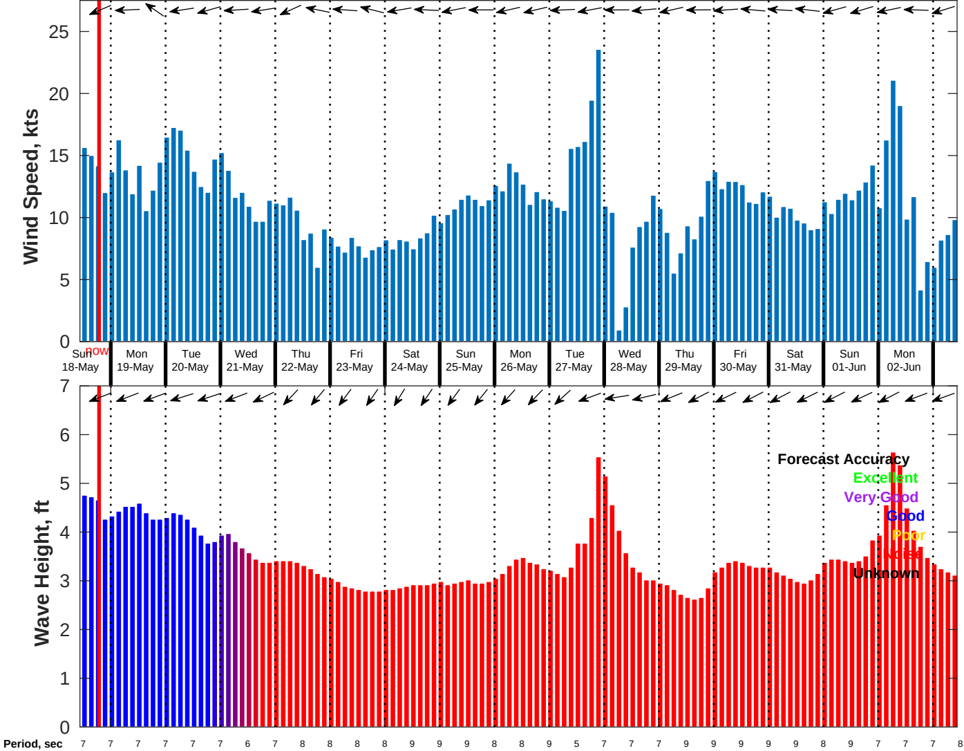
Wind & Wave Forecast for NDBC 52213 from 17-May-2025 11:00:00 to 02-Jun-2025 11:00:00
