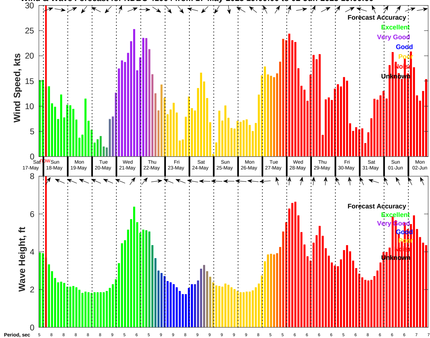
Wind & Wave Forecast for NDBC 41004 from 17-May-2025 19:00:00 to 02-Jun-2025 19:00:00
