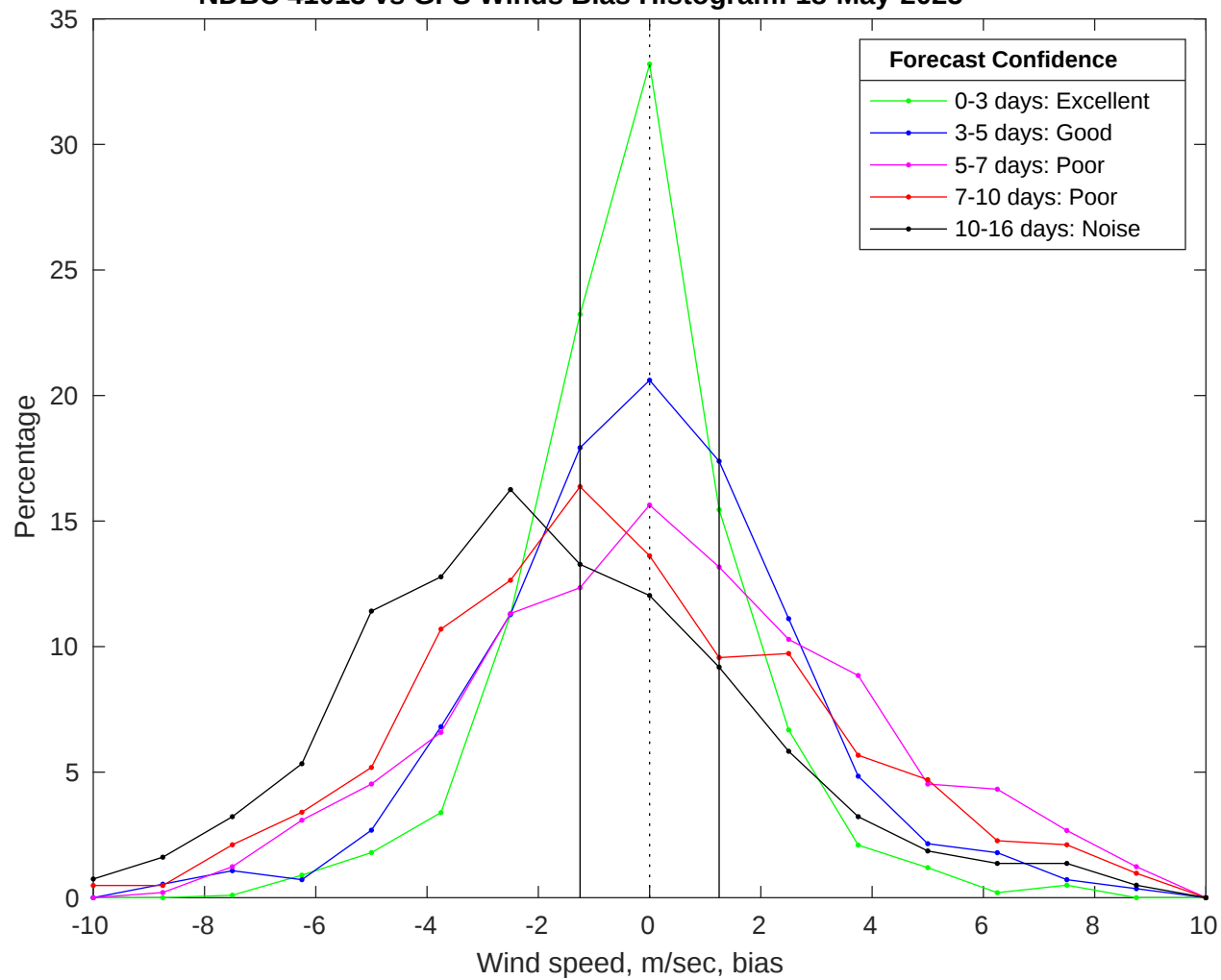
NDBC 41013 vs GFS Winds Bias Histogram: 18-May-2025
