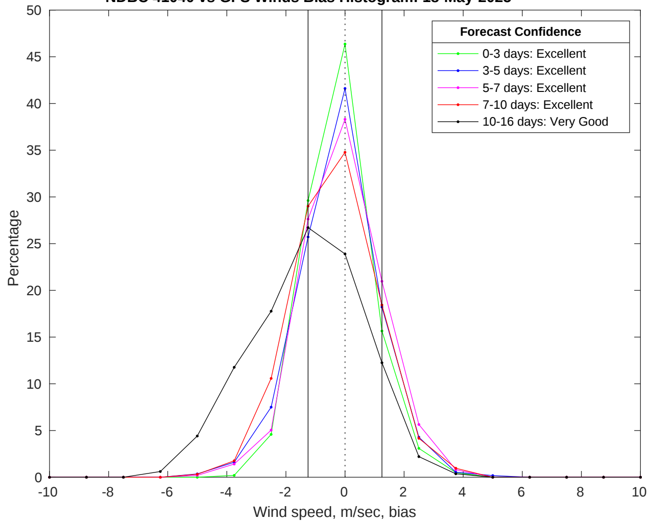
NDBC 41040 vs GFS Winds Bias Histogram: 18-May-2025
