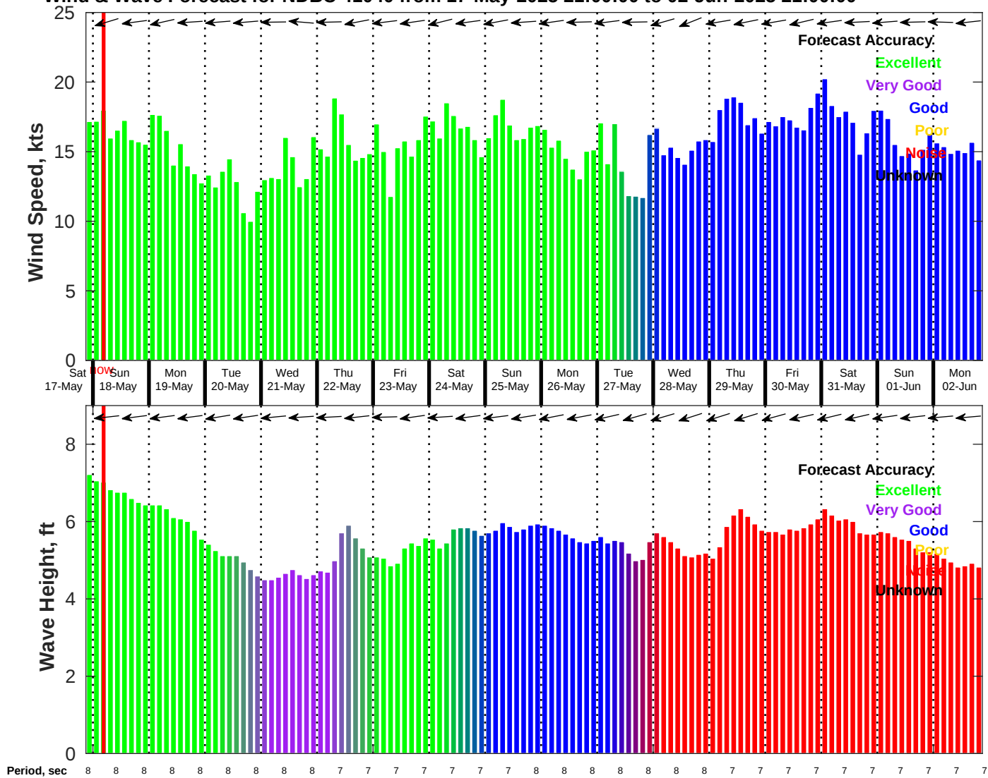
Wind & Wave Forecast for NDBC 41040 from 17-May-2025 21:00:00 to 02-Jun-2025 21:00:00
