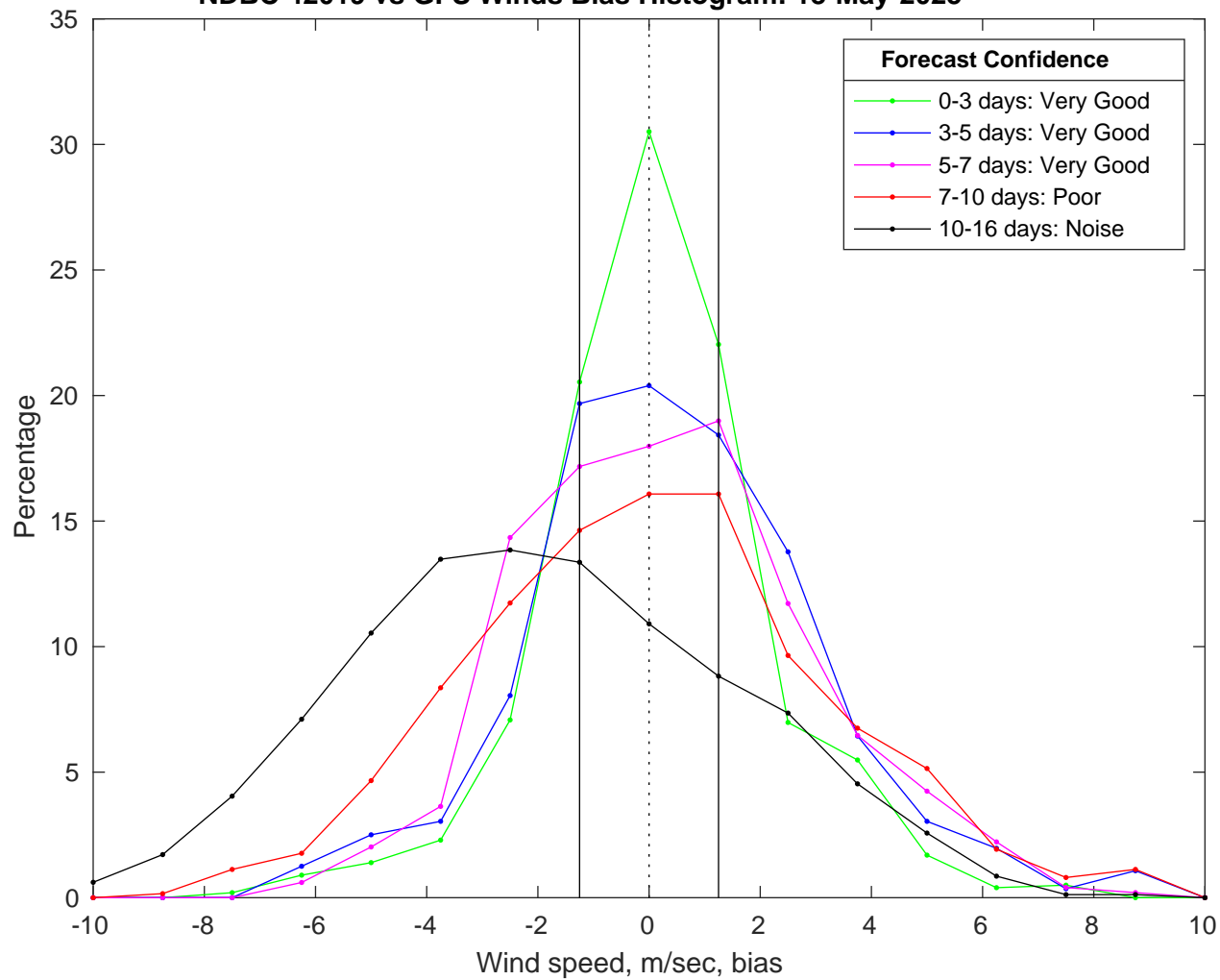
NDBC 42019 vs GFS Winds Bias Histogram: 18-May-2025
